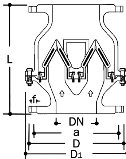
DN 150-400
