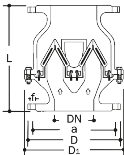
DN 150-400
